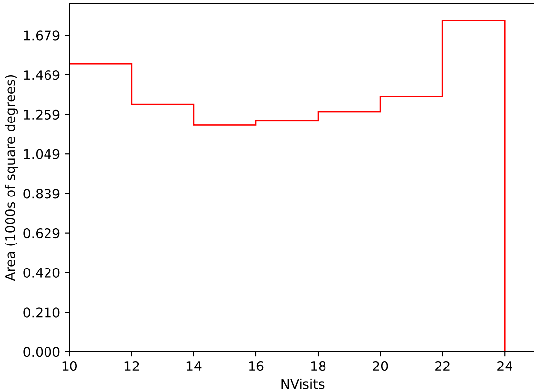
weather_cloudso8v3.4_10yrs Yr 3-4 i band: NVisits
