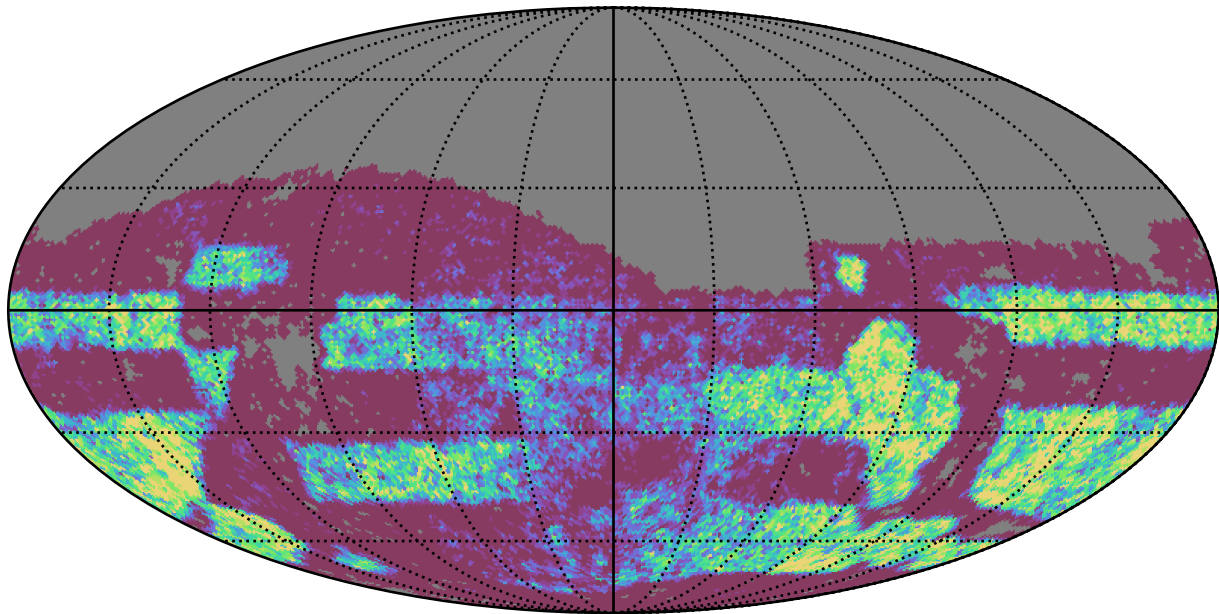
weather_cloudso8v3.4_10yrs Yr 3-4 g band: NVisits
