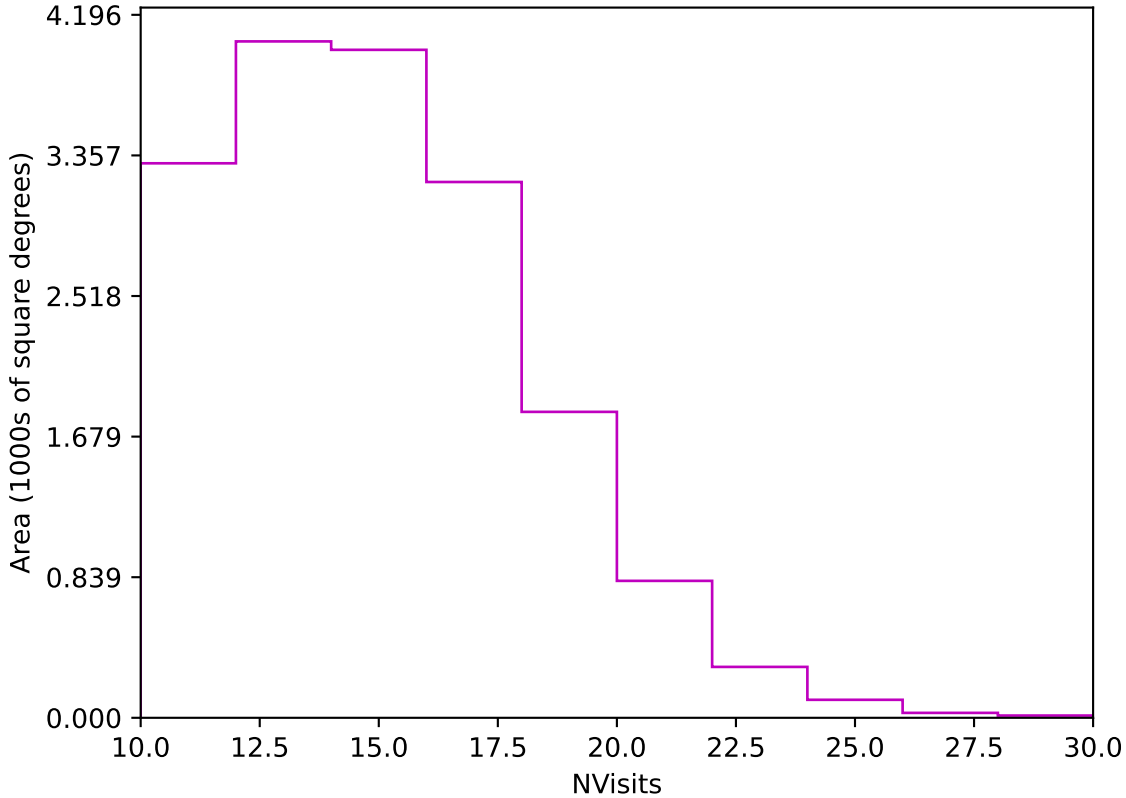
weather_cloudso8v3.4_10yrs Yr 1 z band: NVisits
