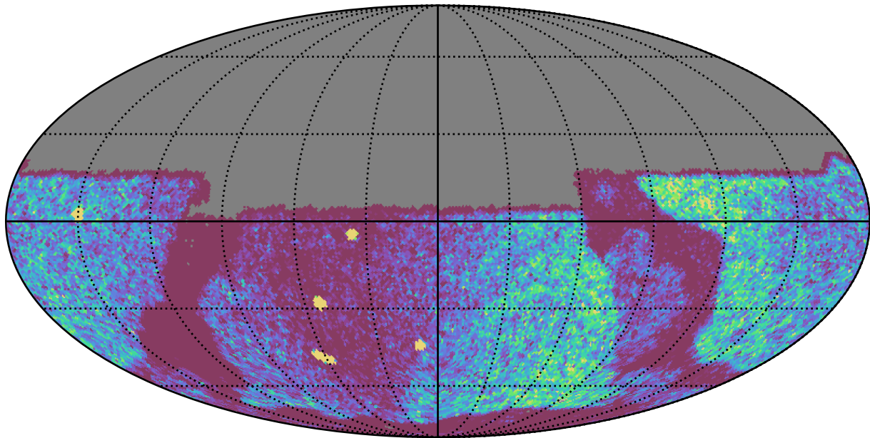
weather_cloudso8v3.4_10yrs Yr 1 y band: NVisits
