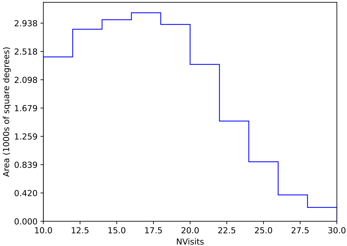
weather_cloudso8v3.4_10yrs Yr 1 y band: NVisits
