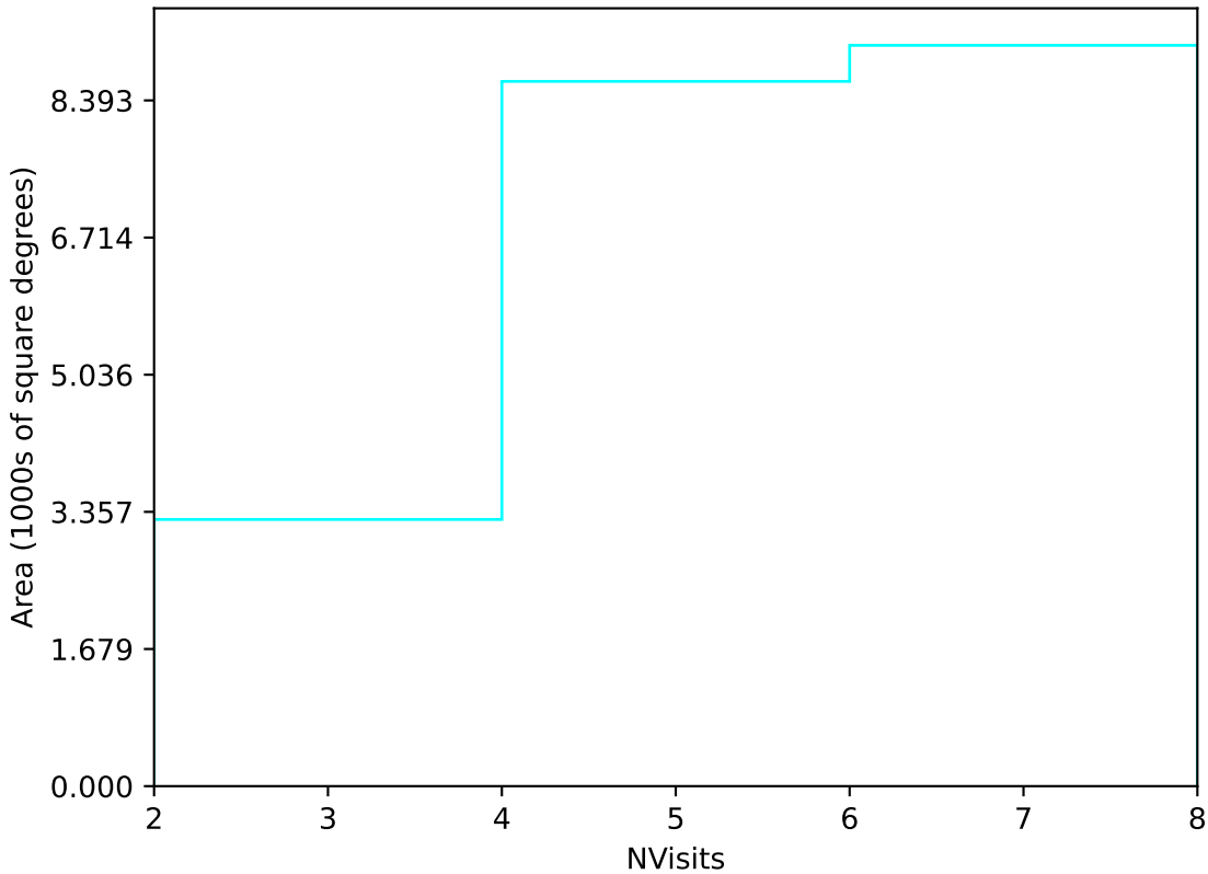
weather_cloudso8v3.4_10yrs Yr 1 u band: NVisits
