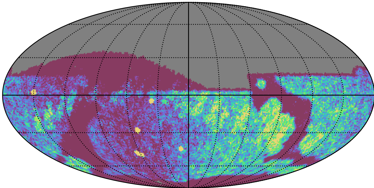
weather_cloudso8v3.4_10yrs Yr 1 r band: NVisits
