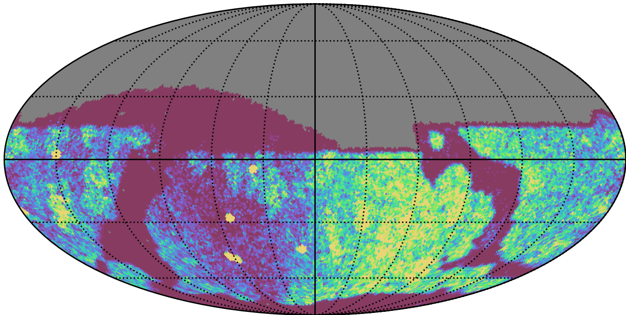
weather_cloudso8v3.4_10yrs Yr 1 i band: NVisits
