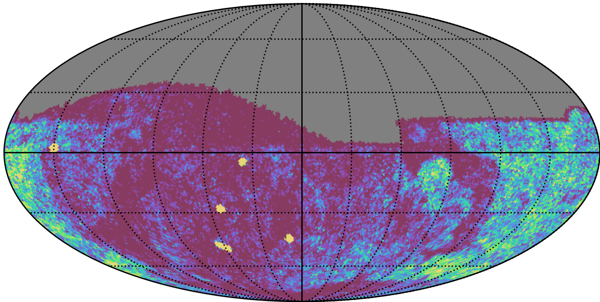
weather_cloudso8v3.4_10yrs Yr 1 g band: NVisits
