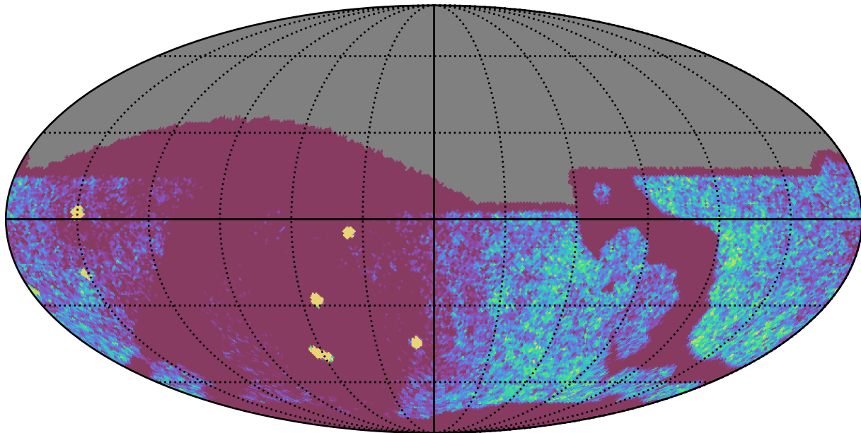
weather_cloudso8v3.4_10yrs Yr 1 all bands: NVisits
