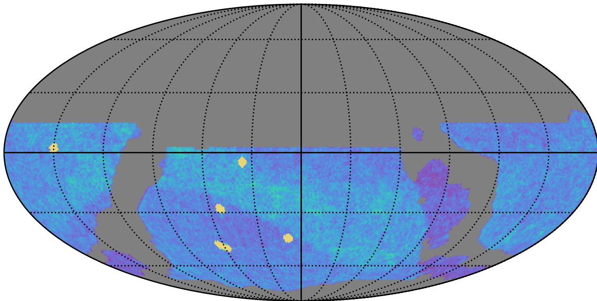
weather_cloudso8v3.4_10yrs WFD z band: NVisits
