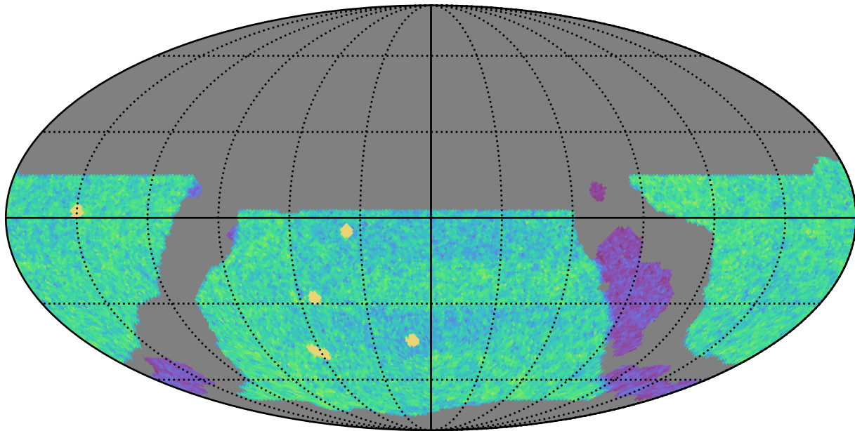
weather_cloudso8v3.4_10yrs WFD u band: NVisits
