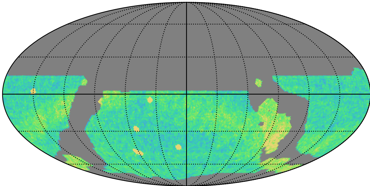
weather_cloudso8v3.4_10yrs WFD r band: NVisits
