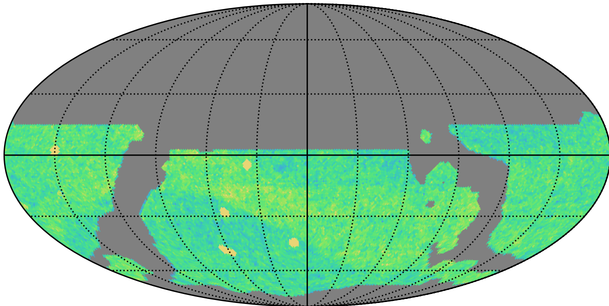
weather_cloudso8v3.4_10yrs WFD i band: NVisits
