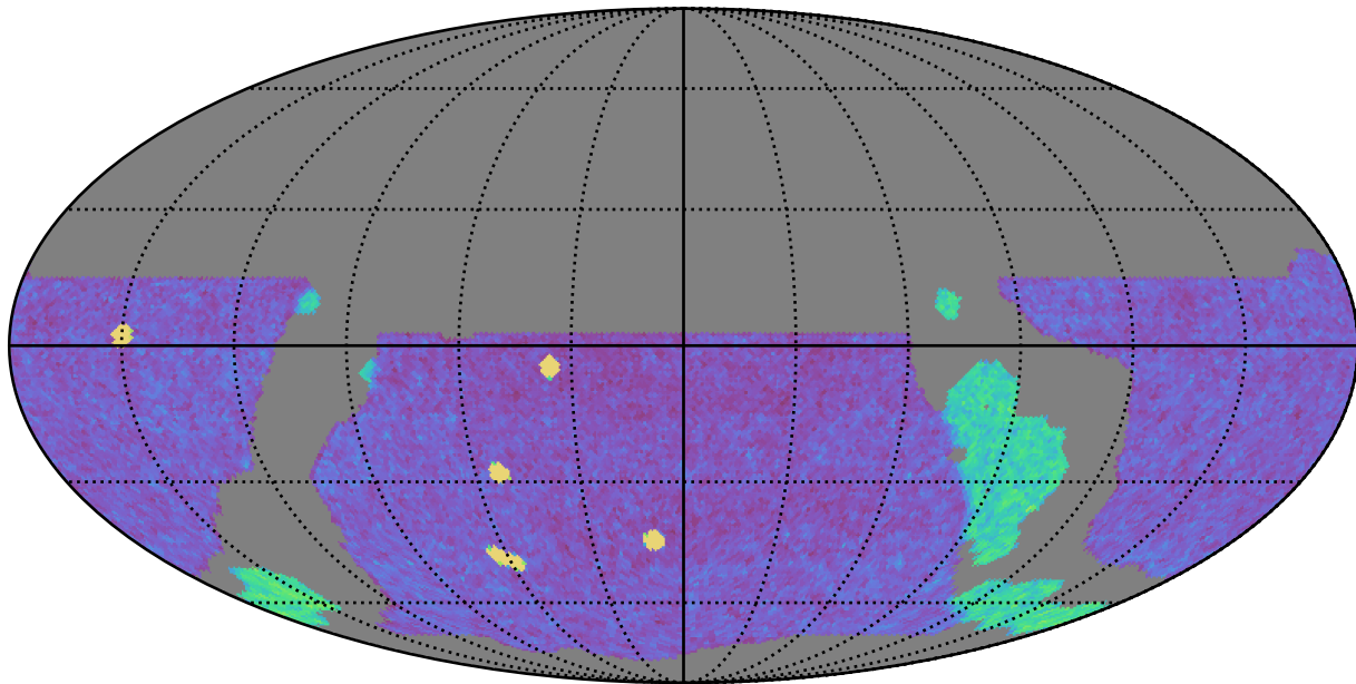
weather_cloudso8v3.4_10yrs WFD g band: NVisits
