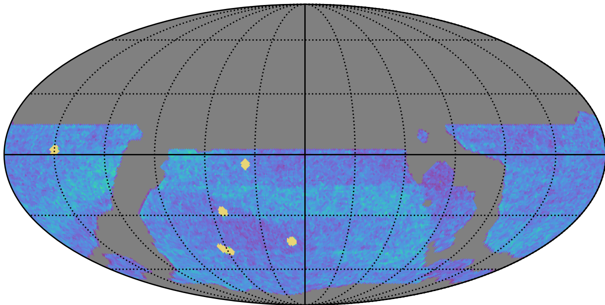
weather_cloudso8v3.4_10yrs WFD all bands: NVisits
