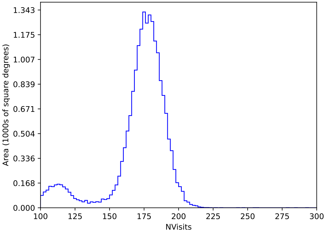
weather_cloudso8v3.4_10yrs All sky y band: NVisits
