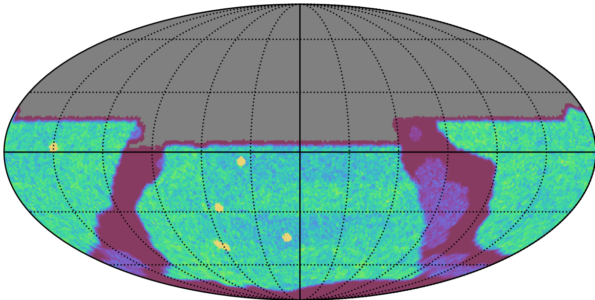
weather_cloudso8v3.4_10yrs All sky u band: NVisits
