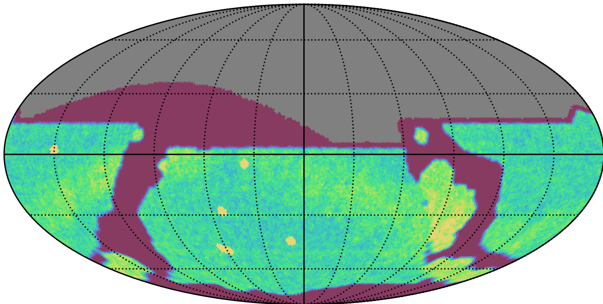
weather_cloudso8v3.4_10yrs All sky r band: NVisits
