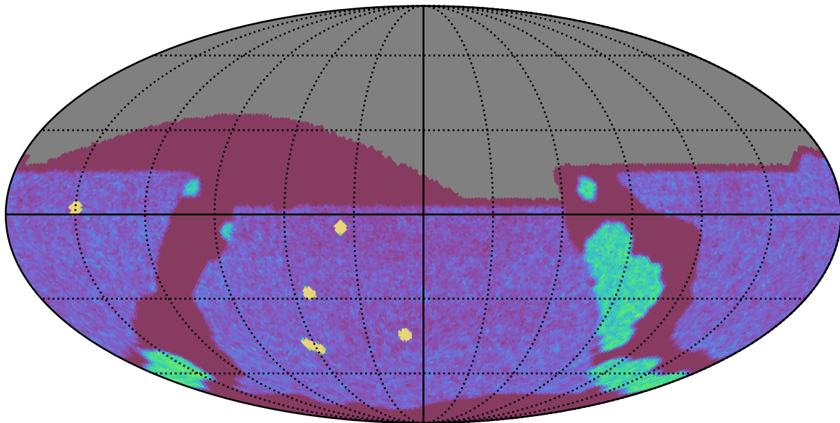
weather_cloudso8v3.4_10yrs All sky g band: NVisits
