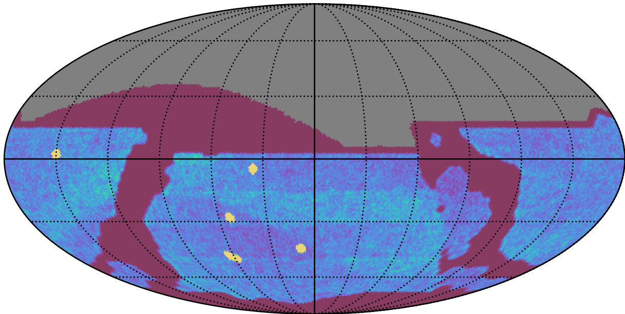
weather_cloudso8v3.4_10yrs All sky all bands: NVisits
