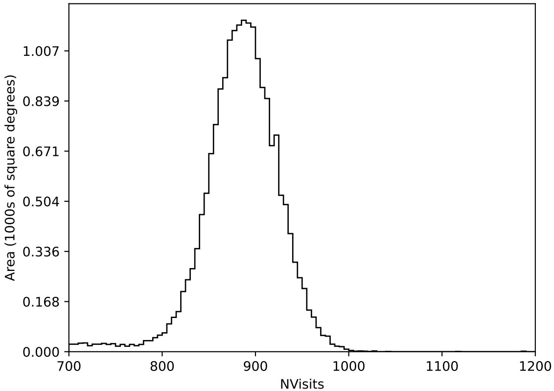
weather_cloudso8v3.4_10yrs All sky all bands: NVisits
