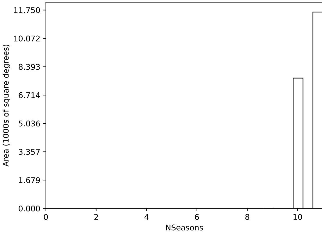
weather_cloudso8v3.4_10yrs WFD all bands: NSeasons
