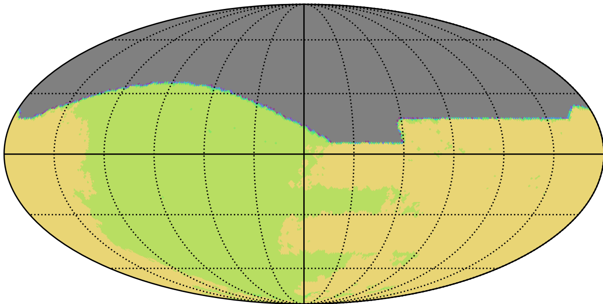
weather_cloudso8v3.4_10yrs All sky all bands: NSeasons
