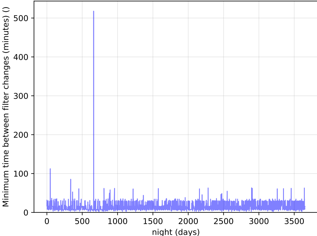
weather_cloudso8v3.4_10yrs Per Night: Minimum time between filter changes (minutes)
