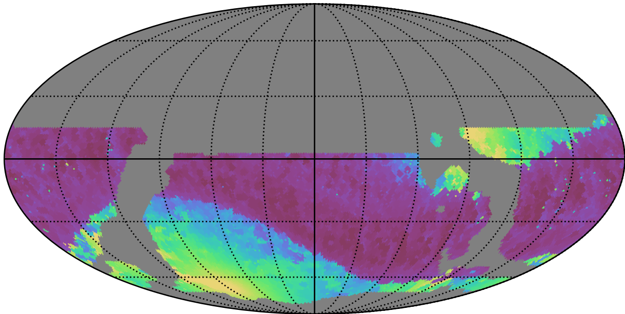
weather_cloudso8v3.4_10yrs WFD z band: Min solarElong
