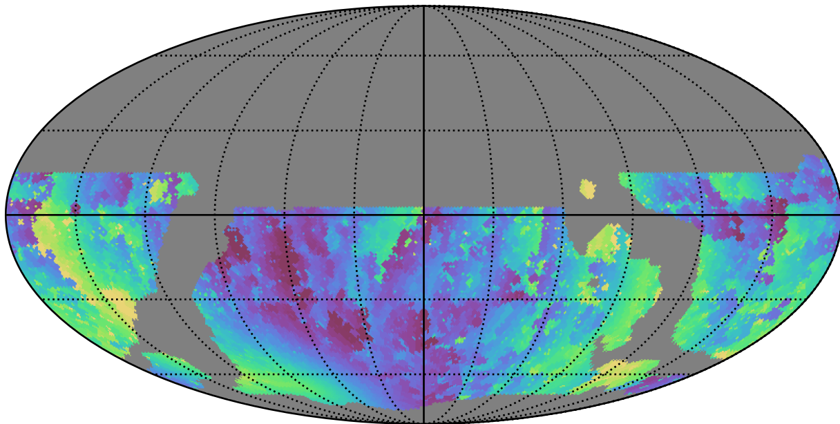
weather_cloudso8v3.4_10yrs WFD u band: Min solarElong
