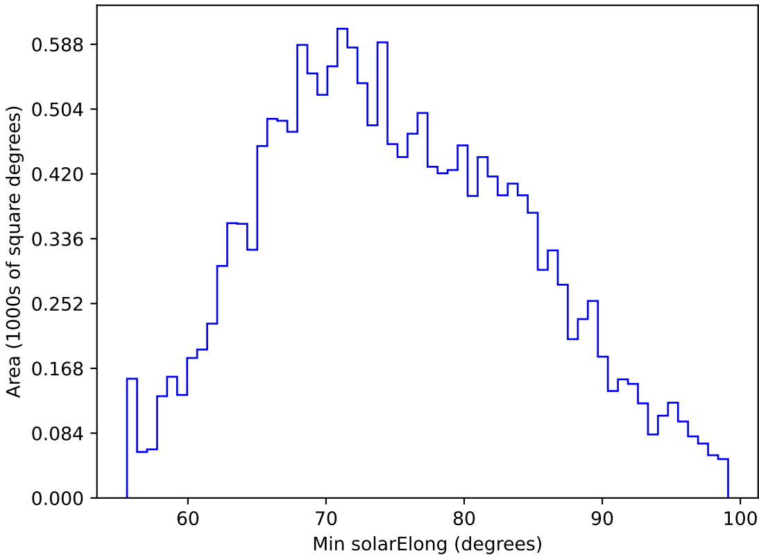
weather_cloudso8v3.4_10yrs WFD u band: Min solarElong
