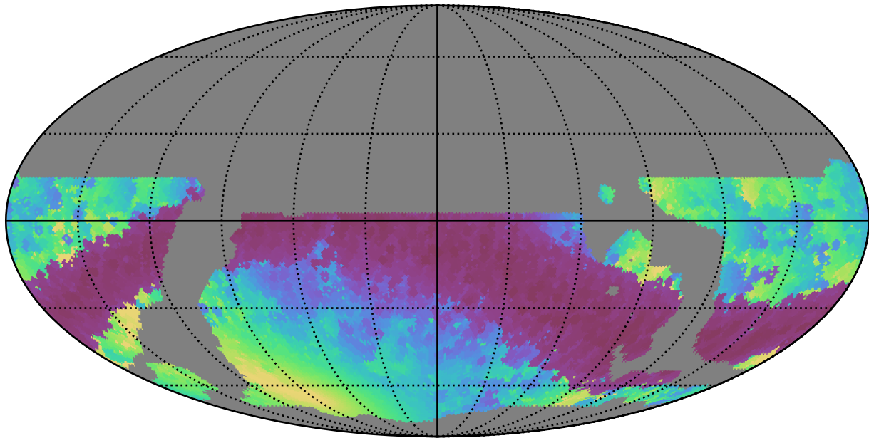
weather_cloudso8v3.4_10yrs WFD r band: Min solarElong
