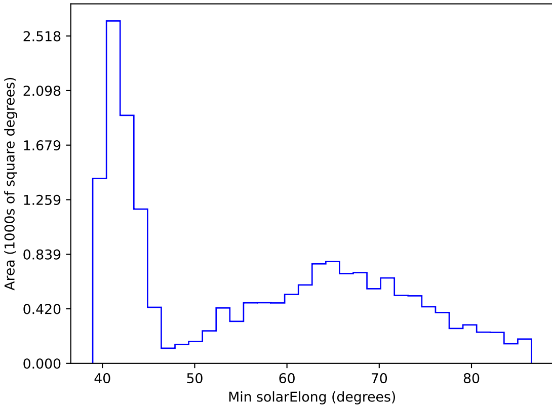
weather_cloudso8v3.4_10yrs WFD r band: Min solarElong
