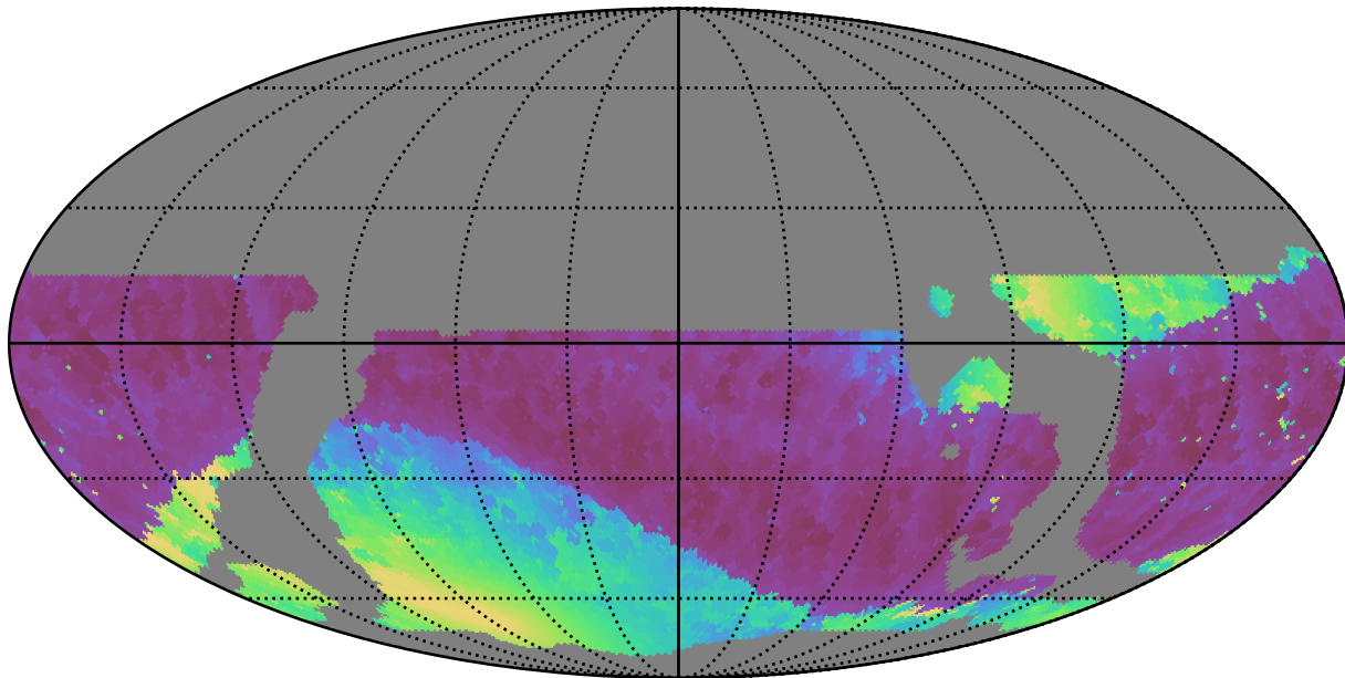
weather_cloudso8v3.4_10yrs WFD i band: Min solarElong
