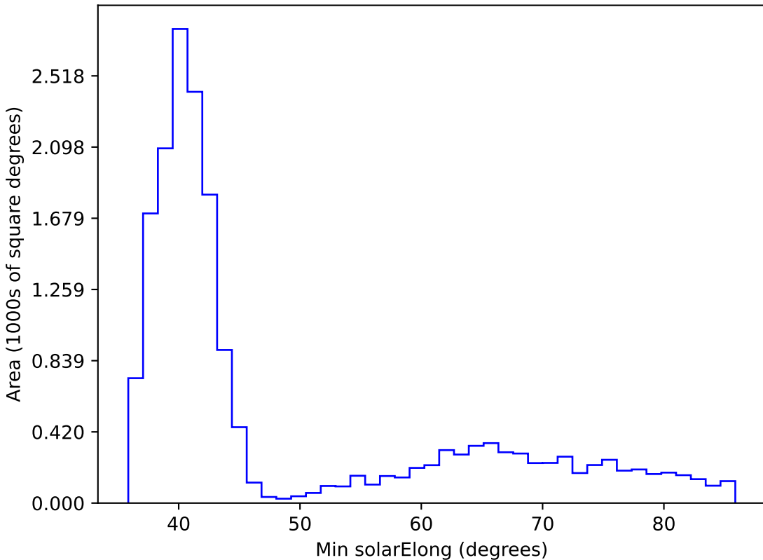
weather_cloudso8v3.4_10yrs WFD i band: Min solarElong
