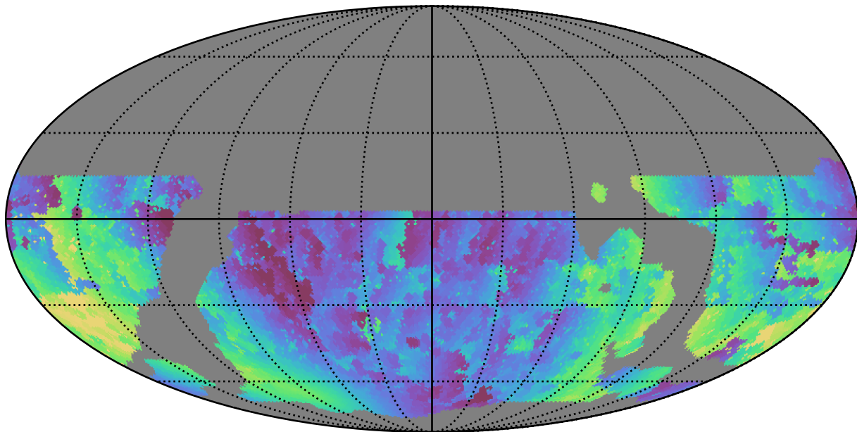
weather_cloudso8v3.4_10yrs WFD g band: Min solarElong
