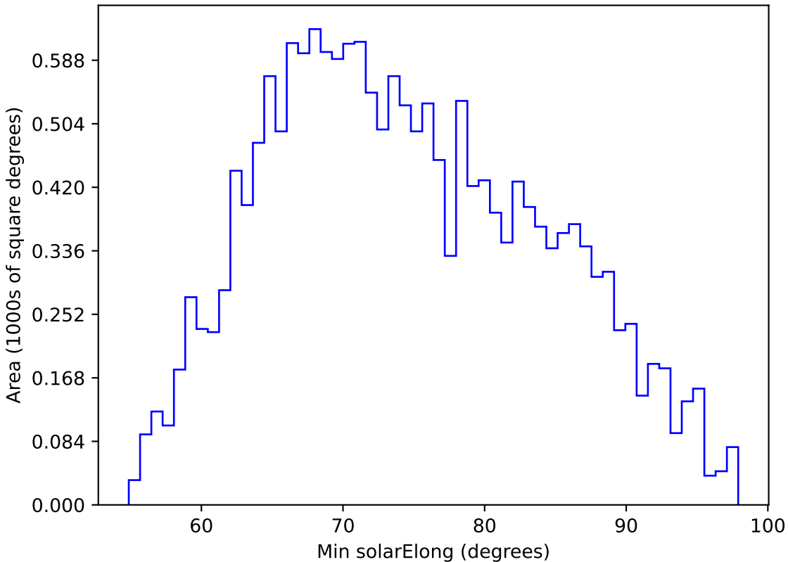
weather_cloudso8v3.4_10yrs WFD g band: Min solarElong
