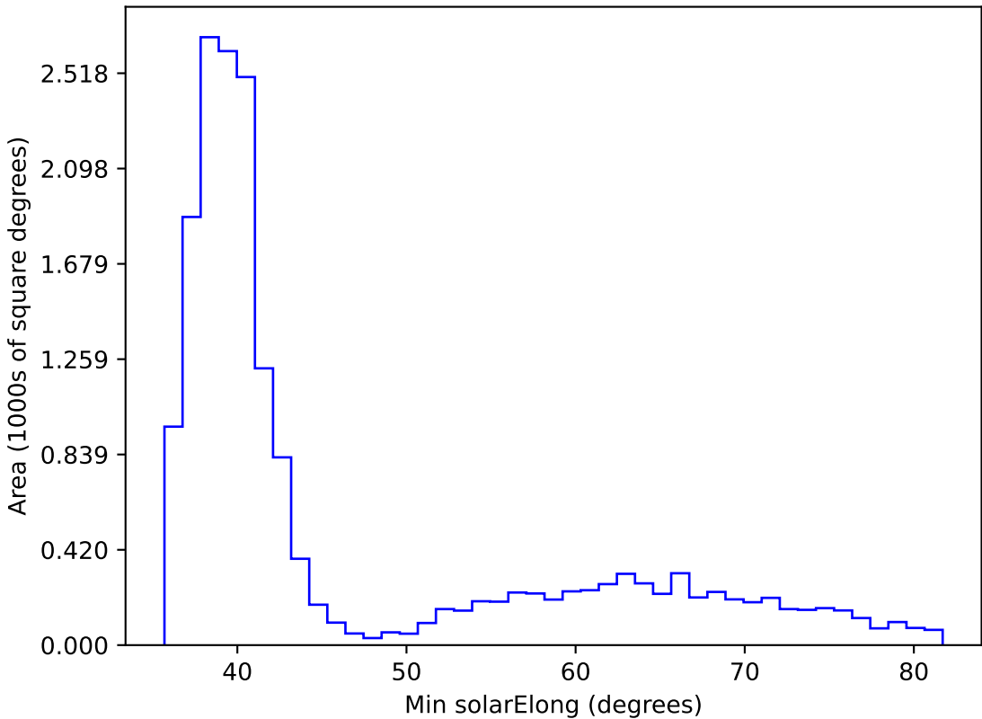
weather_cloudso8v3.4_10yrs WFD all bands: Min solarElong
