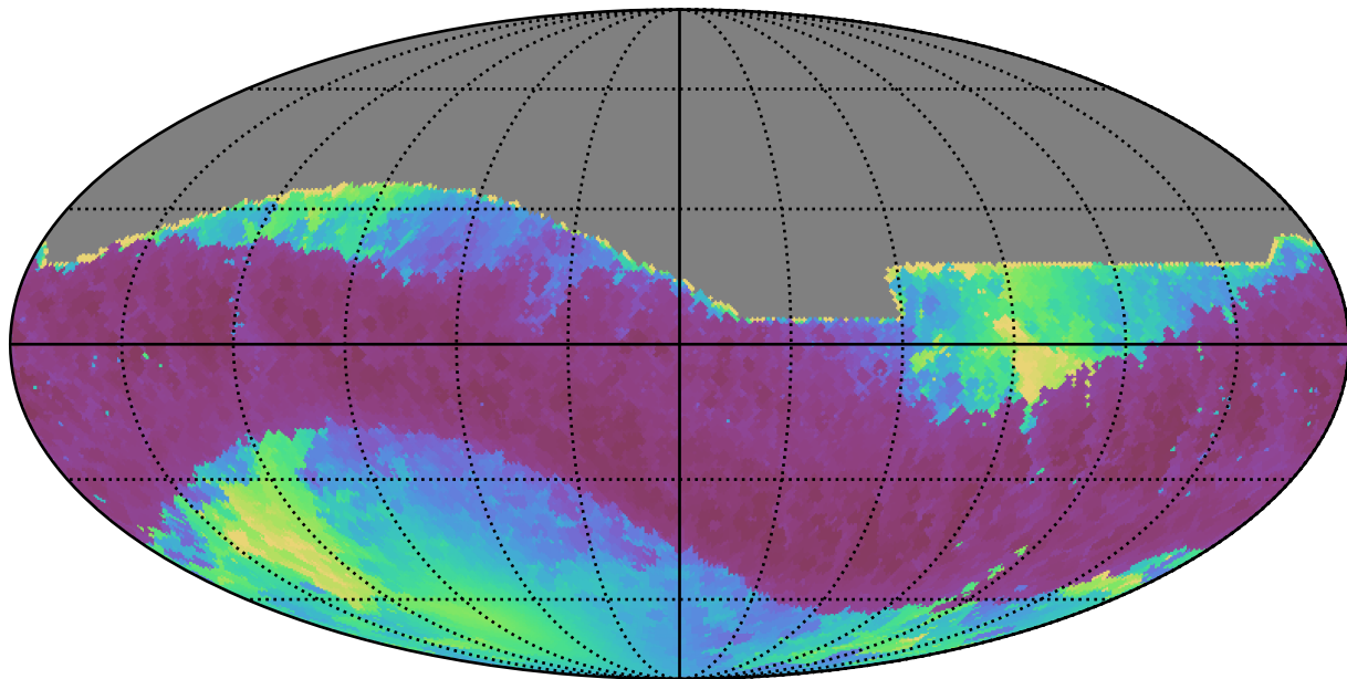
weather_cloudso8v3.4_10yrs All sky z band: Min solarElong
