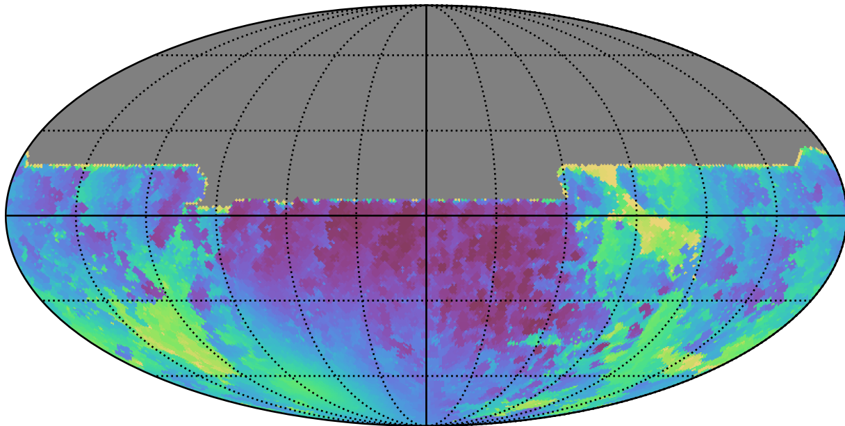
weather_cloudso8v3.4_10yrs All sky y band: Min solarElong
