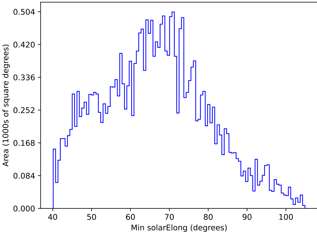
weather_cloudso8v3.4_10yrs All sky y band: Min solarElong
