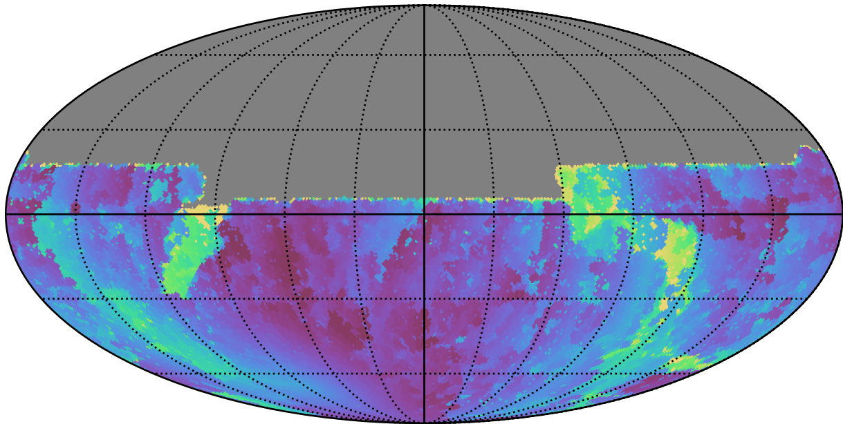
weather_cloudso8v3.4_10yrs All sky u band: Min solarElong
