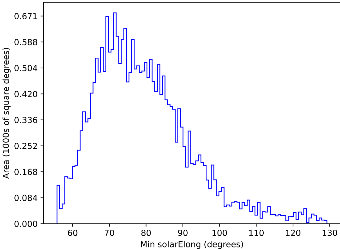
weather_cloudso8v3.4_10yrs All sky u band: Min solarElong
