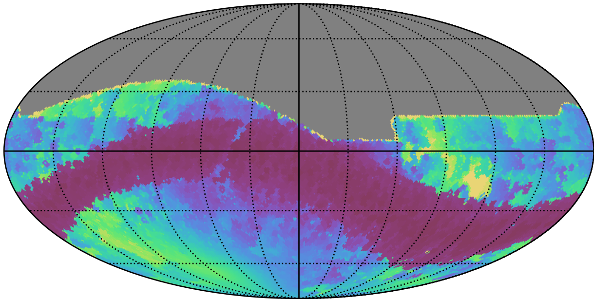
weather_cloudso8v3.4_10yrs All sky r band: Min solarElong
