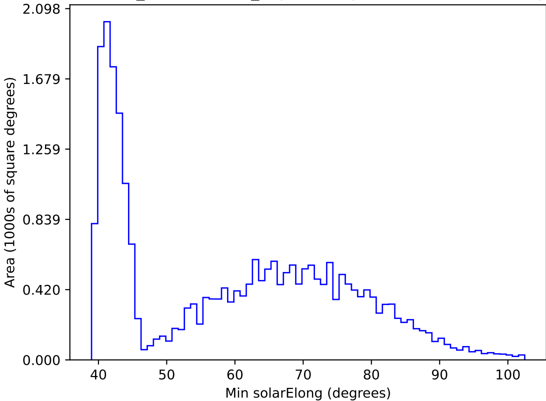
weather_cloudso8v3.4_10yrs All sky r band: Min solarElong
