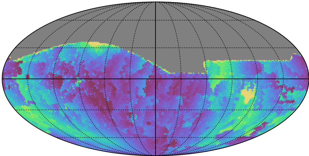
weather_cloudso8v3.4_10yrs All sky g band: Min solarElong
