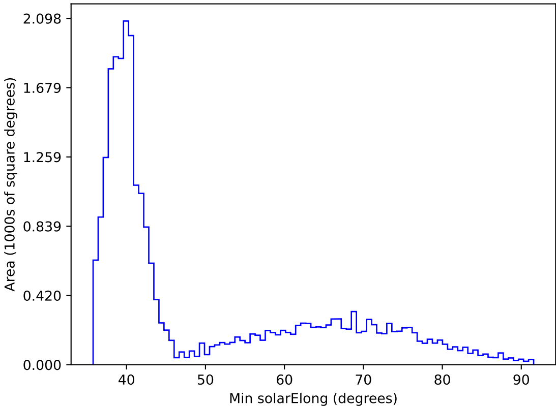
weather_cloudso8v3.4_10yrs All sky all bands: Min solarElong
