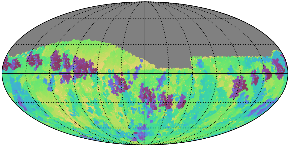
weather_cloudso8v3.4_10yrs Yr 1 z band: Min skyBrightness
