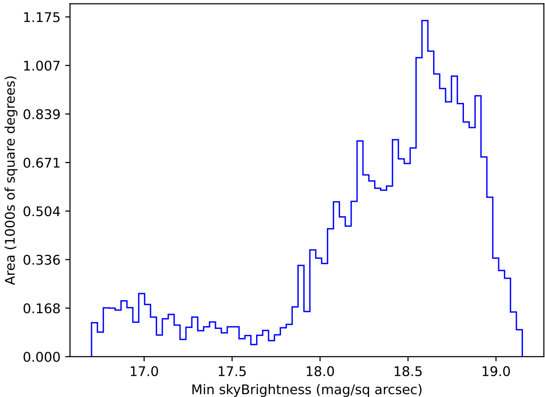
weather_cloudso8v3.4_10yrs Yr 1 z band: Min skyBrightness
