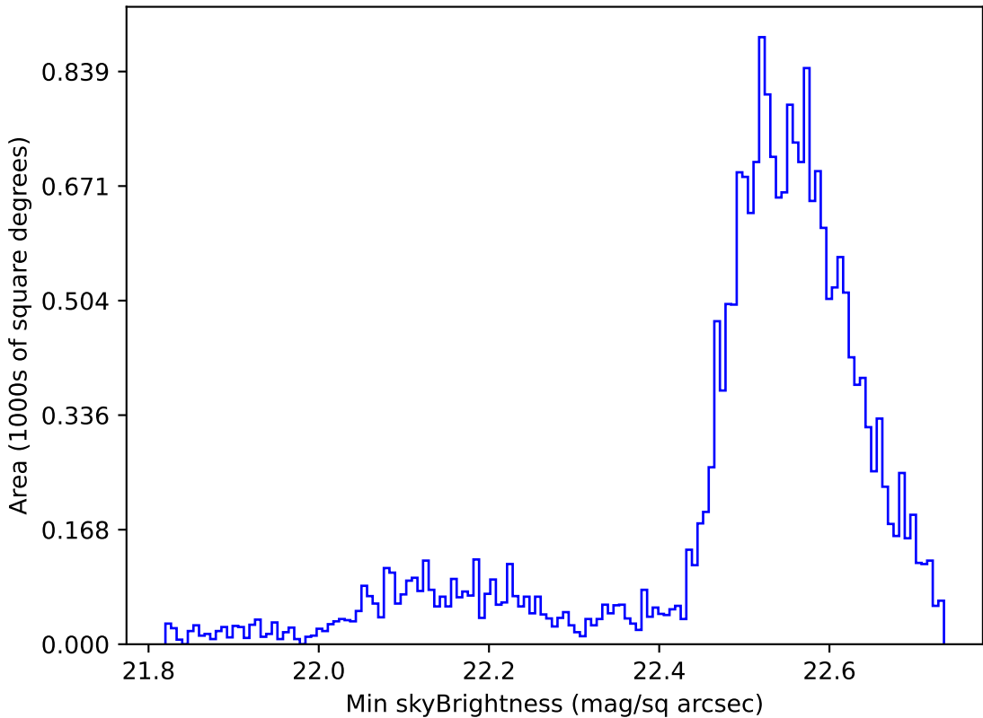
weather_cloudso8v3.4_10yrs Yr 1 u band: Min skyBrightness
