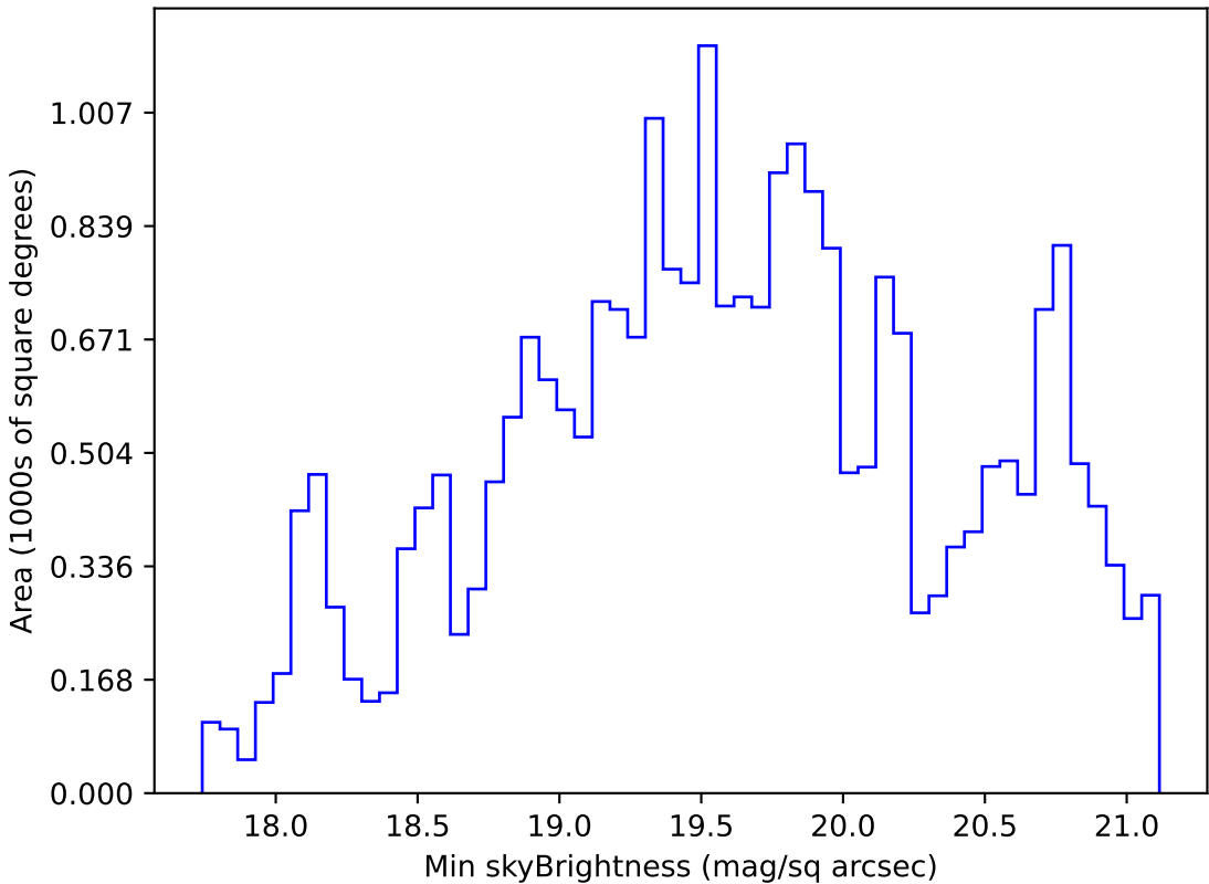
weather_cloudso8v3.4_10yrs Yr 1 r band: Min skyBrightness
