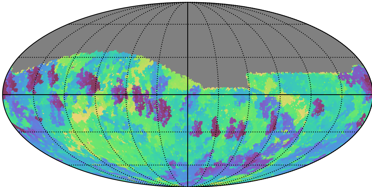
weather_cloudso8v3.4_10yrs Yr 1 i band: Min skyBrightness
