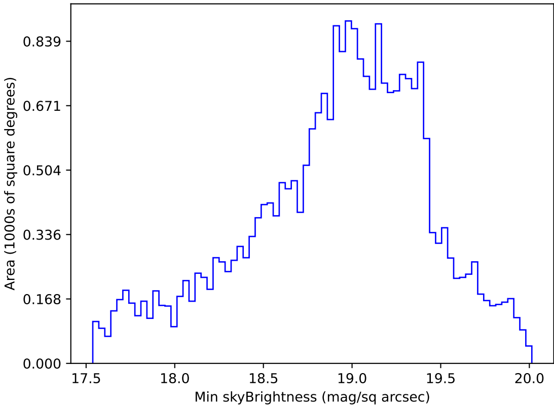
weather_cloudso8v3.4_10yrs Yr 1 i band: Min skyBrightness
